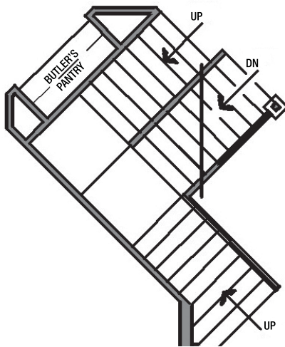
OPEN BASEMENT STAIR OPTION (MAIN LEVEL)
