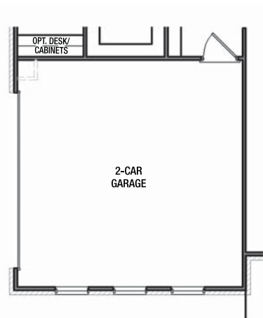
SIDE ENTRY OPTION
